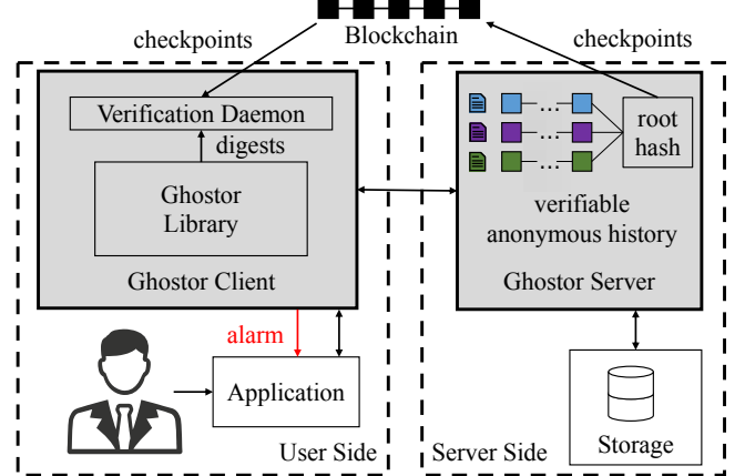
Figure 4: System overview of Ghostor. Shaded areas indicate components introduced by Ghostor.
