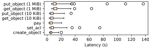
Figure 13: End-to-end latencies of client-side operations
